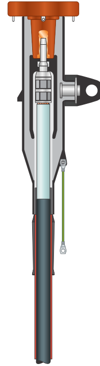
Straight Connector, Type-A
