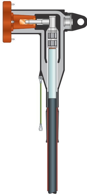
Elbow Connector, Type-A
